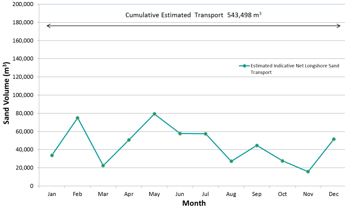
Monthly Estimated Indicative Net Longshore Sand Transport at Letitia Beach January 2015 to December 2015
