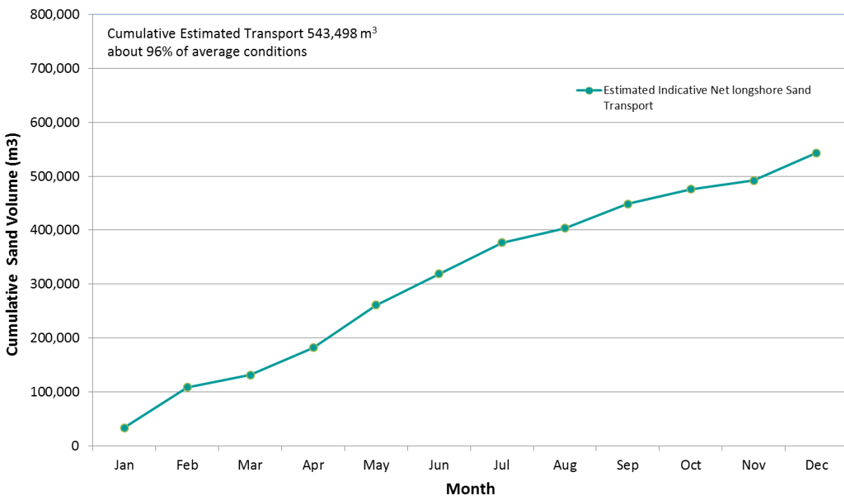
Cumulative Estimated Indicative Net Longshore Sand Transport at Letitia Beach January - December 2015
